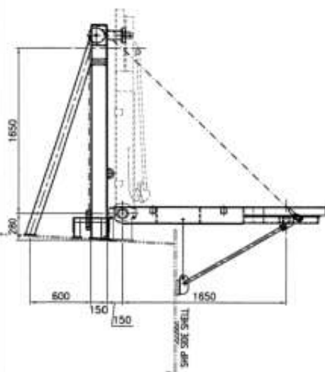
"D" VIEW
