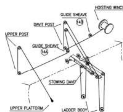
RIGGING DIAGRAM
