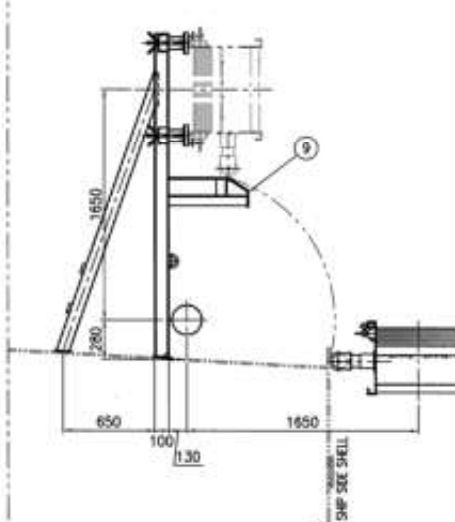
"RA" VIEW
