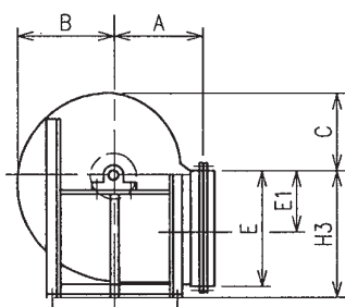
BH - L TYPE
