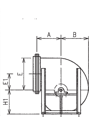
TH - L TYPE
