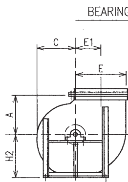
TV - L TYPE
