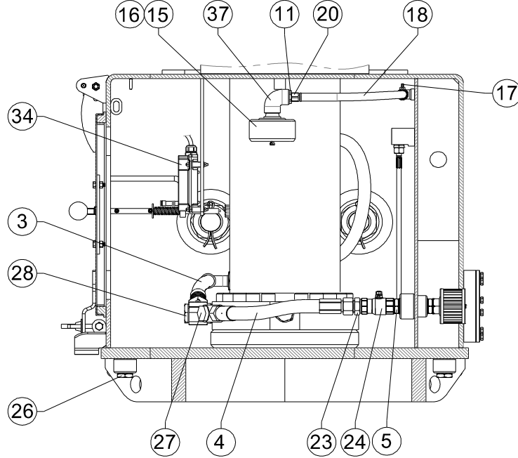
Interior view of the chassis
